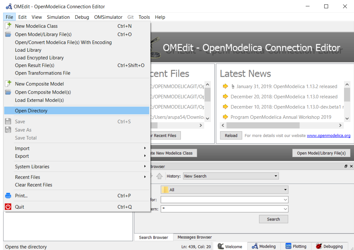
Figure 3.18: open-directory
