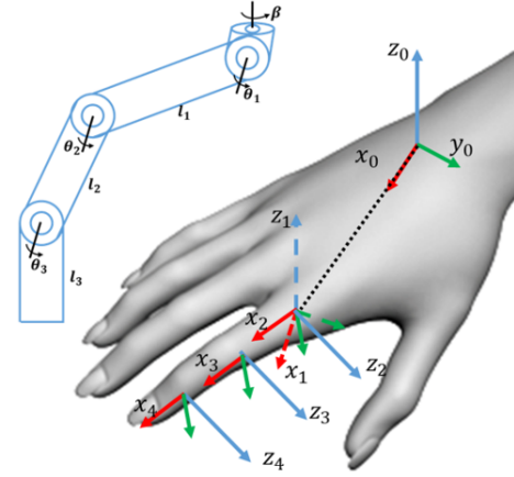
Fig. 5: Frame attachment and the kinematic chain of the index finger, as an example
