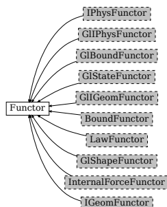
Fig. 32: Inheritance graph of Functor, gray dashed classes are discussed in their own sections: IPhysFunctor , GIIPhysFunctor , GIBoundFunctor , GIStateFunctor , GIGeomFunctor , BoundFunctor , LawFunctor , GShapeFunctor , InternalForceFunctor , IGeomFunctor .
