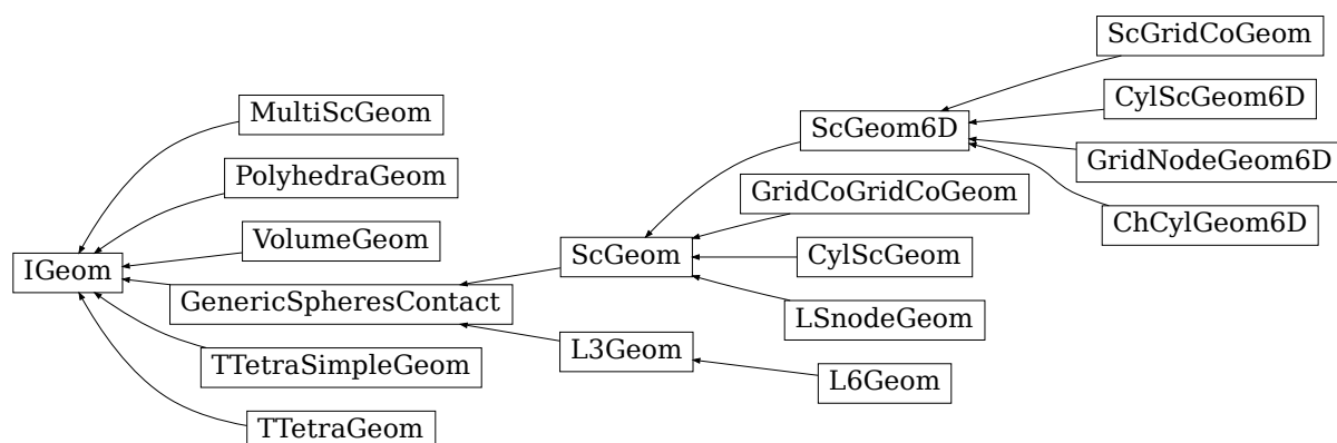
Fig. 23: Inheritance graph of IGeom . See also: ChCylGeom6D , CylScGeom , CylScGeom6D , GenericSpheresContact , GridCoGridCoGeom , GridNodeGeom6D , L3Geom , L6Geom , LSnodeGeom , MultiScGeom , PolyhedraGeom , ScGeom , ScGeom6D , ScGridCoGeom , TTetraGeom , TTetraSimpleGeom , VolumeGeom .
