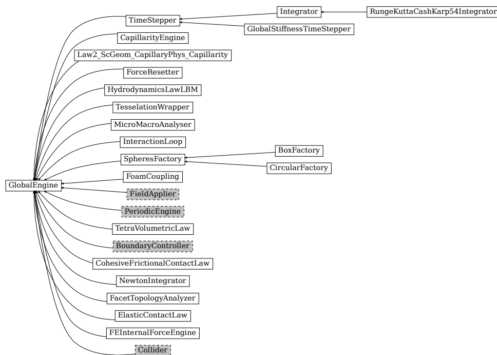
Fig. 25: Inheritance graph of GlobalEngine, gray dashed classes are discussed in their own sections: FieldApplier , PeriodicEngine , BoundaryController , Collider . See also: BoxFactory , CapillarityEngine , CircularFactory , CohesiveFrictionalContactLaw , ElasticContactLaw , FEInternalForceEngine , FacetTopologyAnalyzer , FoamCoupling , ForceResetter , GlobalStiffnessTimeStepper , HydrodynamicsLawLBM , Integrator , InteractionLoop , Law2_ScGeom_CapillaryPhys_Capillarity , MicroMacroAnalyser , NewtonIntegrator , RungeKuttaCashKarp54Integrator , SpheresFactory , TessellationWrapper , TetraVolumetricLaw , TimeStepper .
