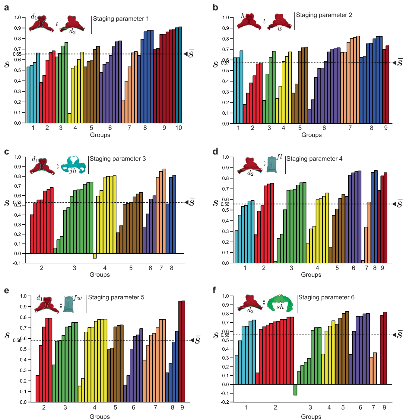
Extended Data Fig. 2 | Silhouette coefficient plot for the different staging parameters explored, classified using k-means and number of groups equal to 10. a-f , Bar graphs showing the silhouette coefficient value ( s ) for each embryo in the collection classified into 10 groups, according to the different staging parameters. The graphs also show the average value ( \bar{s} ), which is maximal for parameter 1. Graphs are color-coded according to the table shown in Fig. 3D. Schemes above the graphs show a representation of staging parameter used.
