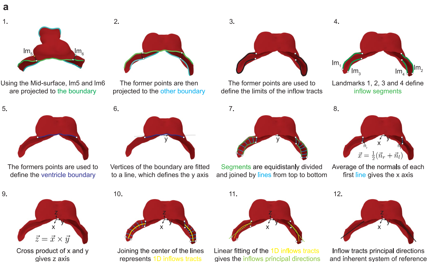
Extended Data Fig. 5 | Proposed algorithm for systematic calculation of a myocardium inherent system of reference and calculation of IFT insertion direction. Steps followed for determining the principal direction of the IFTs and a system of reference based on morphology.
