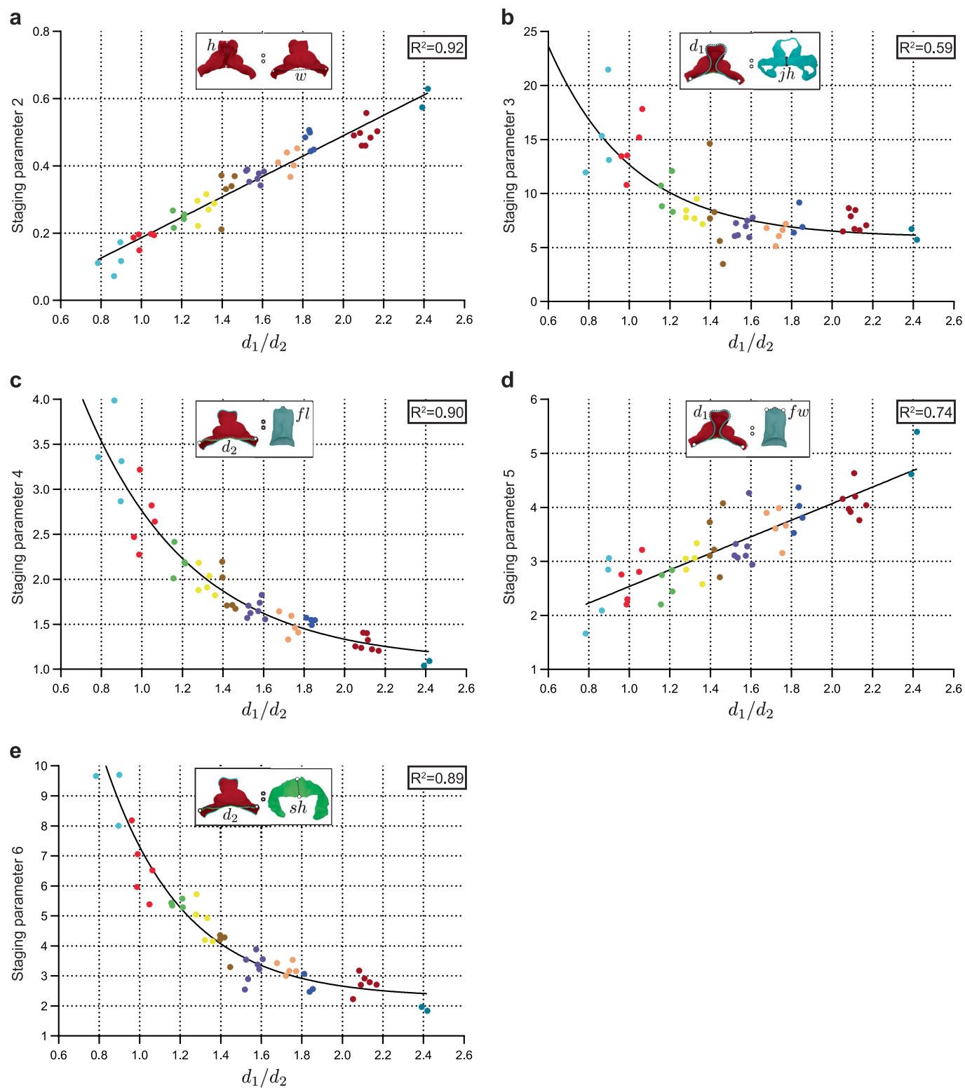
Extended Data Fig. 3 | Correlations between staging parameters unveil tight relationships between the evolution of different morphometric aspects during heart development. a, b, c, d, e, Plots show the correlation of staging parameters 2-6 versus staging parameter 1, d_1/d_2 .
