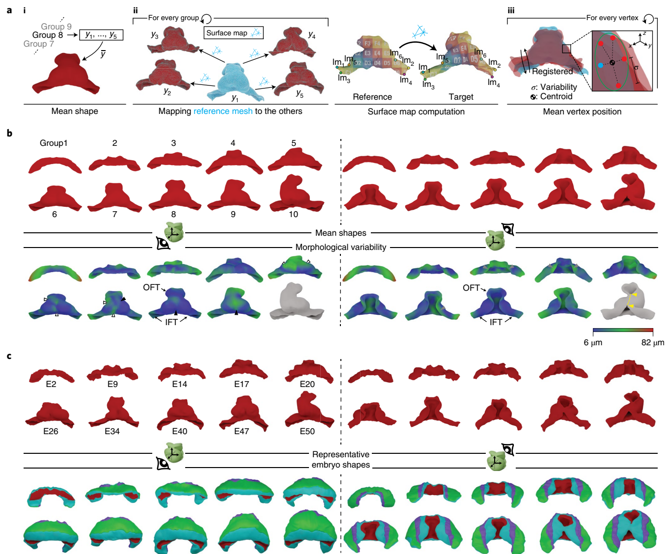
Fig. 4 | MSG and morphological variability. a , Illustration of the concept of mean shape for staging group 8 (i) and workflow for obtaining a mean shape and local variability estimation for each staging group (ii). In ii, the left shows the process of surface map computation. The blue shape represents the mesh of the reference specimen of the group. The arrows represent the surface mapping from the reference specimen mesh to all others in the staging group. The right shows the working principle of the surface map computation. The landmarks (lm) identify corresponding locations in the reference and target mesh. Shapes of the group after rigid registration to the reference mesh are also shown (iii). Every vertex in the reference mesh (blue dot) has a corresponding point on the other shapes (red dots). b , Calculated myocardium mean shapes for every staging group. The two top rows show the mean shapes from ventral (left) and dorsal (right) views. The two bottom rows show the same mean shapes color coded according to the morphological variability calculated for each vertex. The shape in gray indicates that the low number of specimens at this stage precludes variability calculation. The yellow dotted line and arrows represent the cut trajectory to achieve genus 0 topology in dorsally closed hearts (Methods). Arrowheads indicate the regions of higher variability in medial ventricular regions (solid) and lateral ventricular regions (open). c , Representative specimens of each group. Top, ventral and dorsal view of the myocardium shape. Bottom, ventral and dorsal views of the pericardial tissues of the representative embryos.
