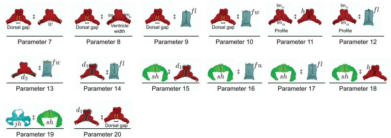
Extended Data Fig. 1 | Additional parameters explored for staging. Schematic representation of additional parameters explored for the staging system.
