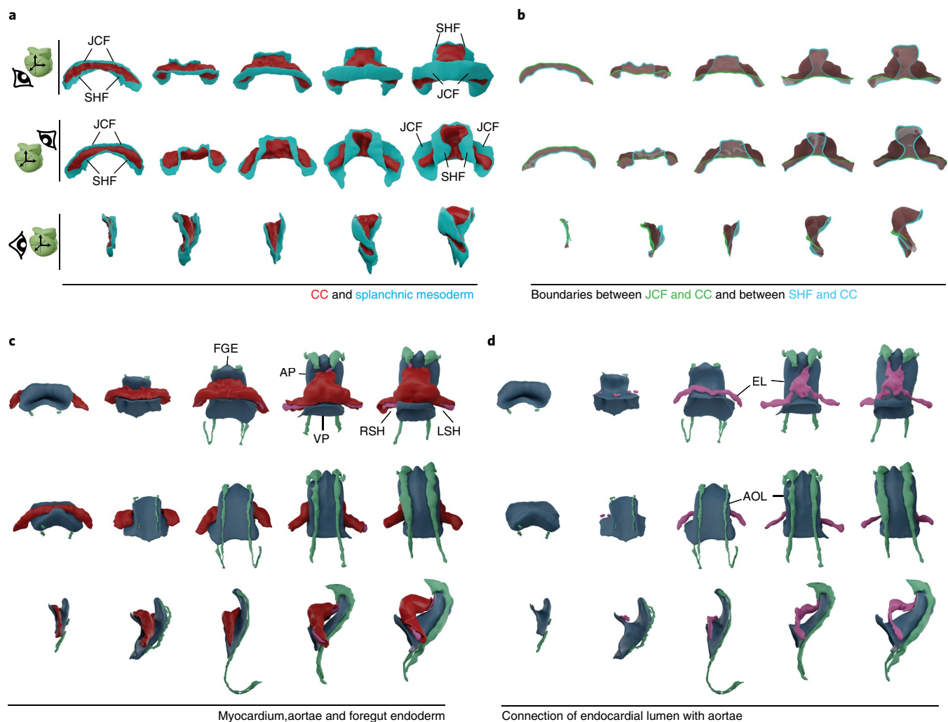
Fig. 2 | Observation of qualitative morphometric aspects of heart tube morphogenesis. a , Ventral, dorsal and lateral views of five specimens that are subjectively ordered according to developmental time. Splanchnic mesoderm is represented in blue, and differentiated myocardium is represented in red. The dorsal view shows the progressive dorsal closure of the heart tube and the medial expansion of the SHF. b , Limits of the myocardial differentiated domain depicted on the edges of the myocardium midsurface. The green line represents the boundary between the juxta-cardiac field and the myocardium. The blue line represents the boundary between the myocardium and the SHF. c , Morphology of the myocardium together with the foregut endoderm and the circulatory system lumen. The different lengths of the aortae seen in the three older specimens are due to variable imaging depth. d , Gradual development of the circulatory system in parallel to the foregut endoderm invagination. The ventral view shows the progressive formation of the endocardial lumen, and the lateral view shows the progressive formation of the aortic lumen along the dorsal surface of the foregut endoderm. Abbreviations: JCF, juxta-cardiac field; FGE, foregut endoderm; AP, arterial pole; VP, venous pole; EL, endocardial lumen; AOL, aortic lumen; LSH, left sinus horn; RSH, right sinus horn.
