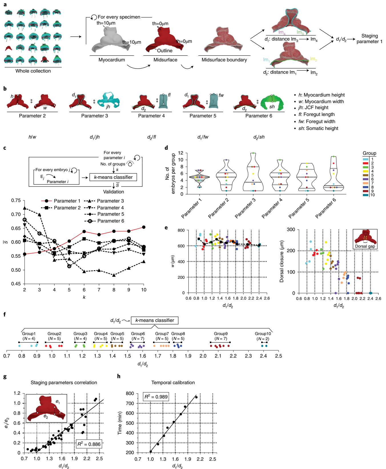
Fig. 3 | Establishment of a morphometric staging system. a , Schematic representation for the calculation of staging parameter 1. lm, landmark; th, thickness. b , Schematic representation of five additional staging parameters. c , Top, workflow for evaluating staging parameters by means of the average silhouette coefficient ( \bar{s} ). Bottom, graph showing the evolution of \bar{s} as a function of the number of groups for every staging parameter. d , Violin plots showing the distribution of specimens in each cluster ( N=10 clusters) for the six selected staging parameters. e , Scatter plots showing myocardium width (left) and dorsal gap width (right) as a function of d_1/d_2 . f , Plot showing the final classification of the collection in 10 groups according to d_1/d_2 . g , Correlation between d_1/d_2 and the staging parameter applied to live-imaging data ( e_1/e_2 ). h , Temporal calibration of the progression of the d_1/d_2 values.
