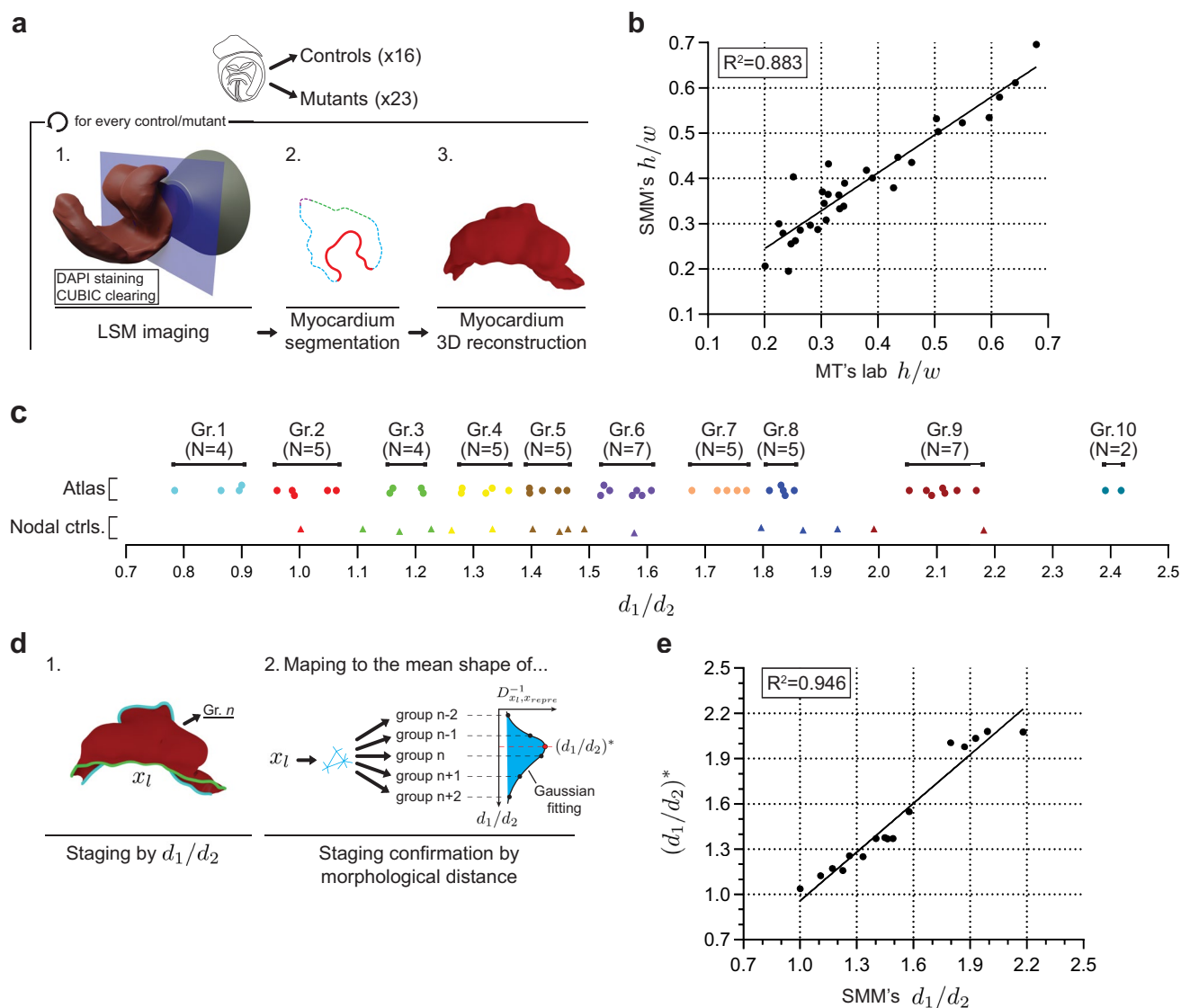
Extended Data Fig. 9 | Pipeline for staging the specimens from the study of Nodal loss of function. a , Steps taken for the image acquisition and segmentation of the Nodal mutant and control specimen series. b , Correlation between the h/w staging parameter independently measured in the SMM and MT labs. c , Mapping of the d_1/d_2 values measured in SMM's control specimen collection. d , Procedure for the morphological mapping of the SMM's control specimen collection to the atlas MSG collection. e , Correlation between the experimentally determined d_1/d_2 parameter and the predicted d_1/d_2 obtained from the morphological mapping of the SMM's control specimen collection to the atlas MSG collection.
