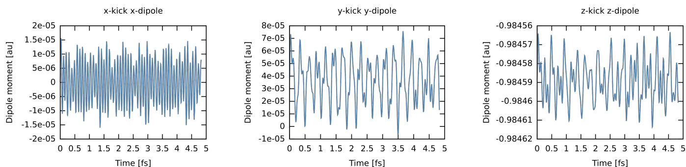
Water Gas-Phase 6-31G/TD-PBE0 Kick Excitation Dipole Moments
