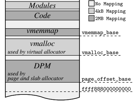
Figure 1: Virtual memory layout of the x86_64 Linux kernel.
