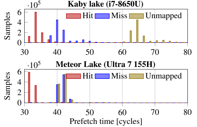
Figure 7: Prefetch timings of 4 kB pages.
