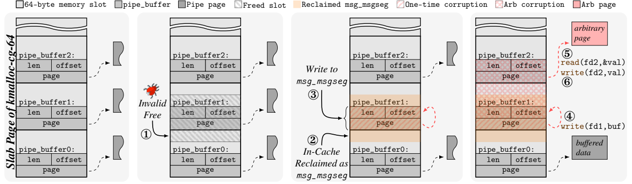
Figure 9: The exploit technique uses an IF and the known location of this slab page to obtain an arbitrary r/w. Initially, the IF ① frees a memory slot containing pipe_buffer1. In-cache reclaiming of this slot ② as a msg_msgseg enables corrupting pipe_buffer1 to point to its physical page ③. Writing to with fd1 ④ corrupts pipe_buffer2, while ⑤/⑥ allows arbitrary r/w.
