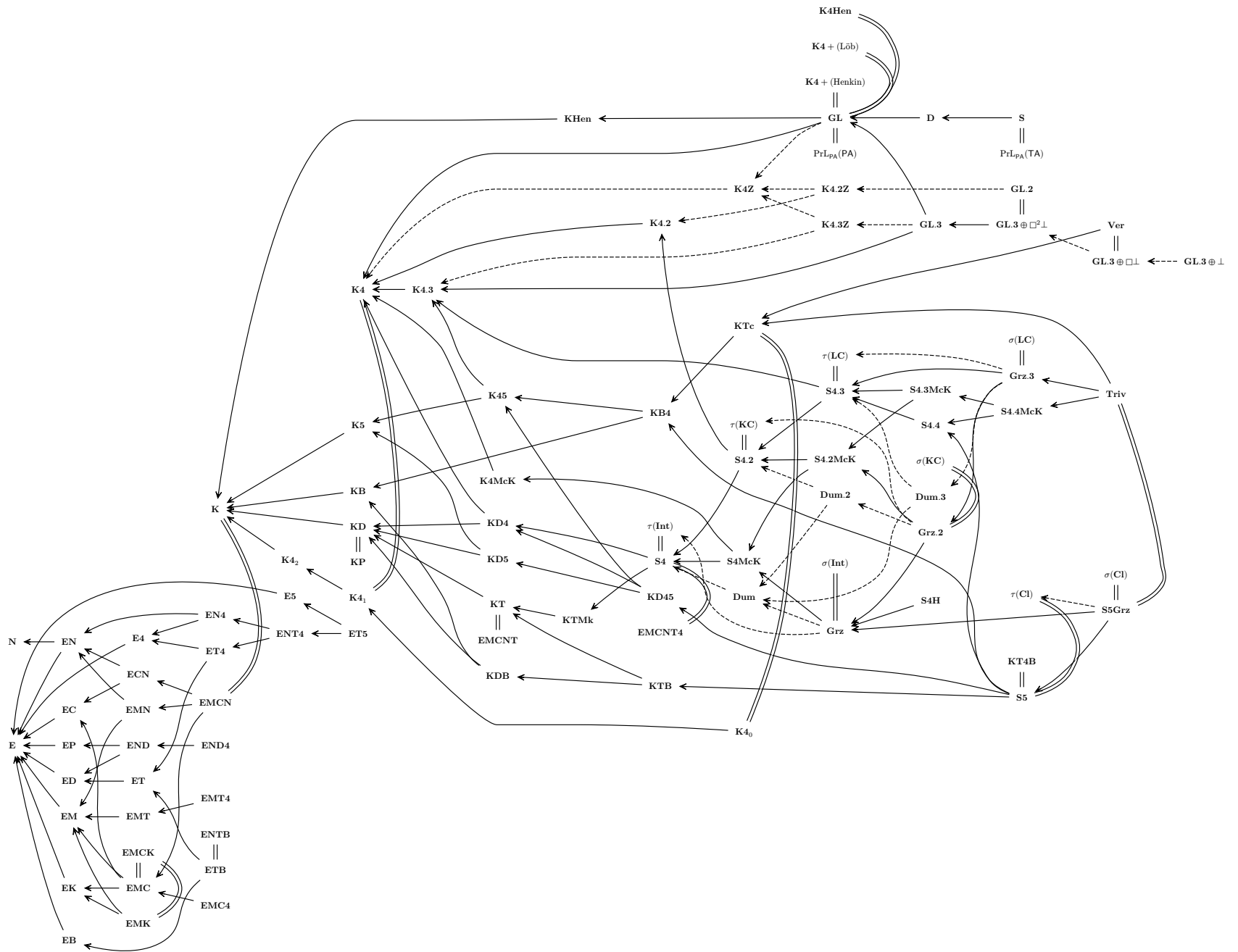
Modal Logic Zoo
