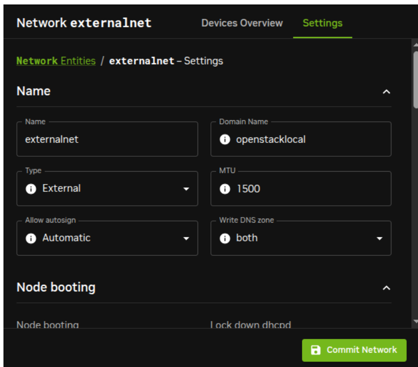
Figure 3.7: Network Settings For External Network
