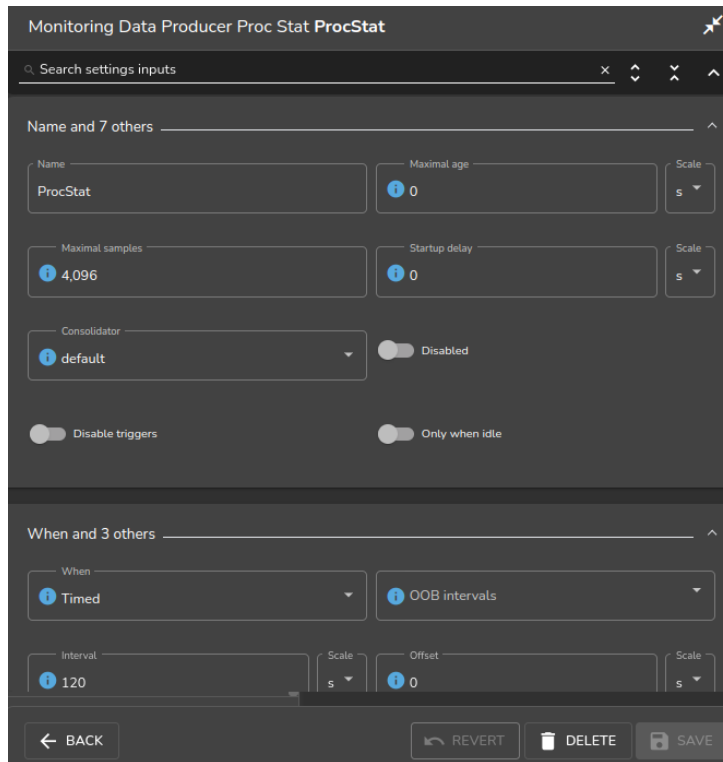
Figure 10.11: Base View Monitoring Configuration Data Producer: ProcStat
