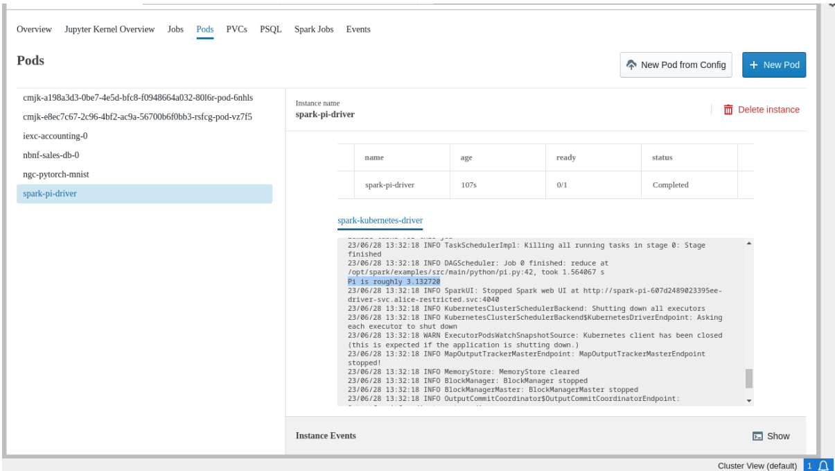
Figure 16.31: Jupyter Kubernetes Operators Manager: pods tab Spark example execution status
