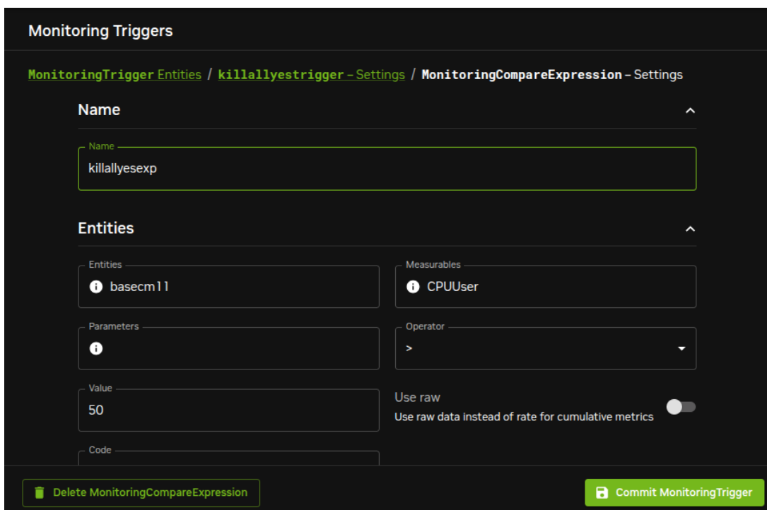
Figure 10.4: Base View Monitoring Configuration: Setting An Expression
