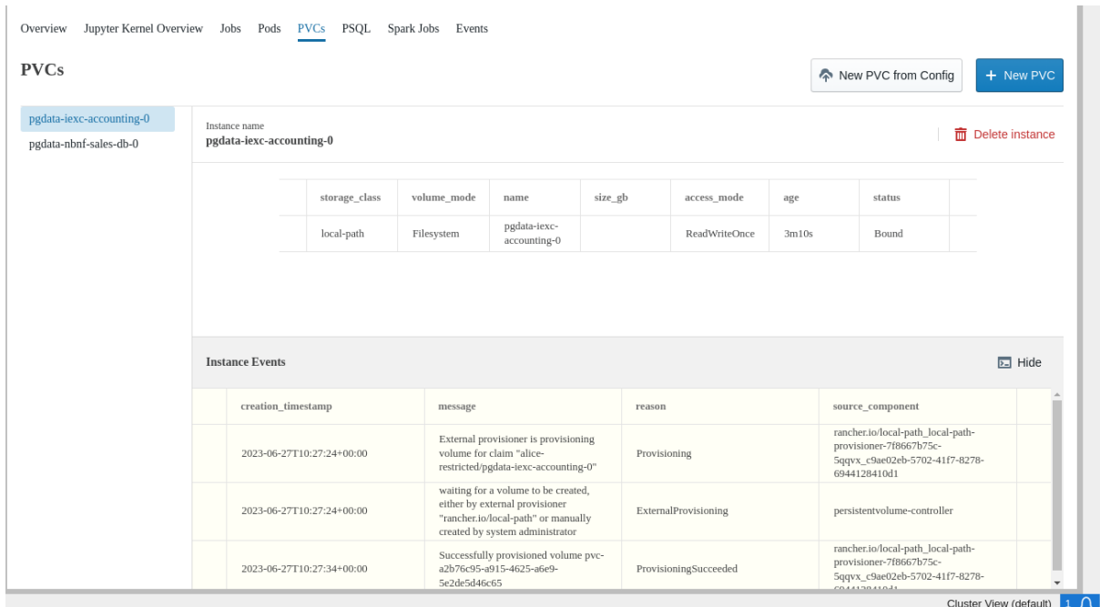
Figure 16.24: Jupyter Kubernetes Operators Manager: PVCs overview tab
