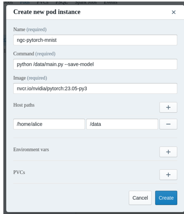
Figure 16.23: Jupyter Kubernetes Operators Manager: pod creation
