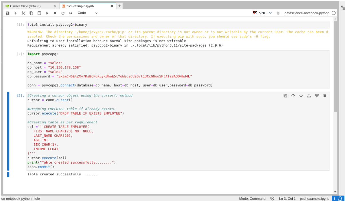
Figure 16.27: Jupyter Kubernetes Operators Manager: PSQL notebook
