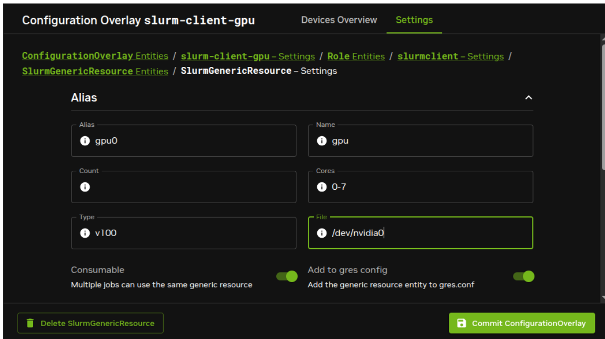
Figure 7.20: Base View access to NVIDIA GPU configuration options
