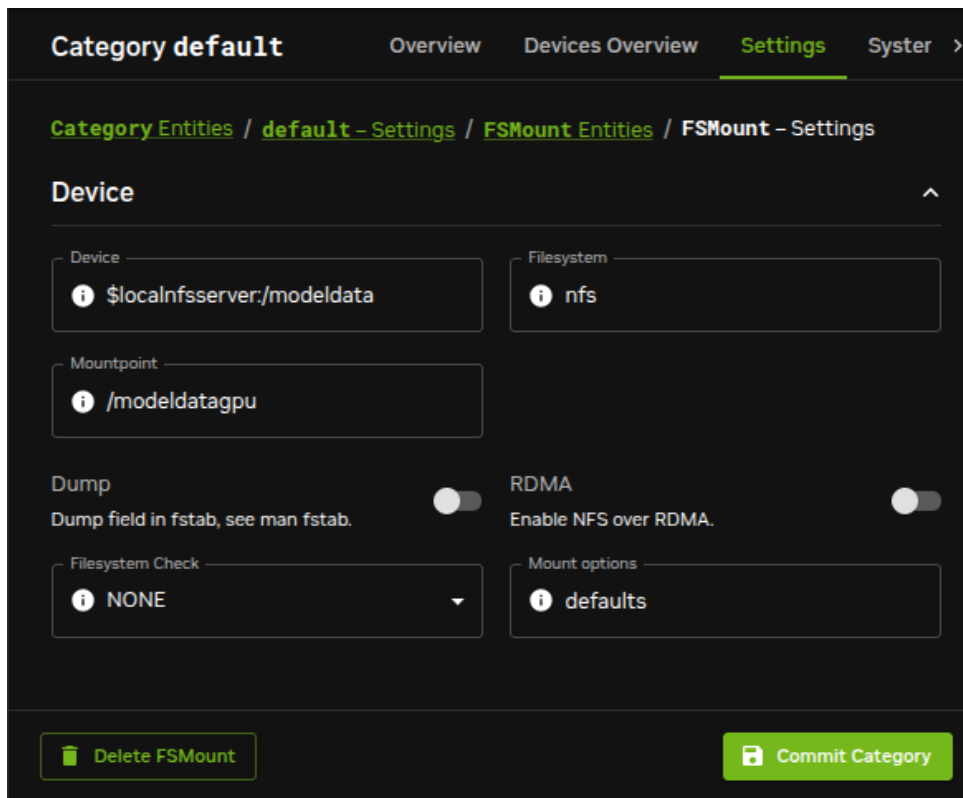
Figure 3.21: Setting up NFS mounts on a node category using Base View
