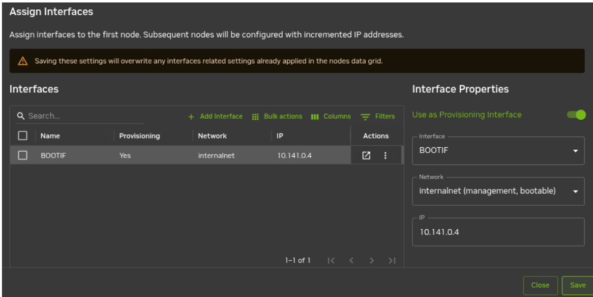
Figure 5.22: Node Creation Wizard: Adding Interface Settings For Bulk Assignment
