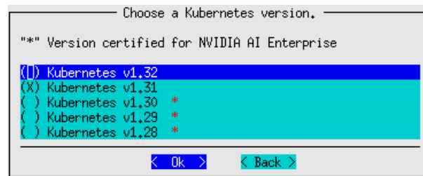
Figure 4.1: Kubernetes setup TUI session (section 4.2.6): version selection screen
