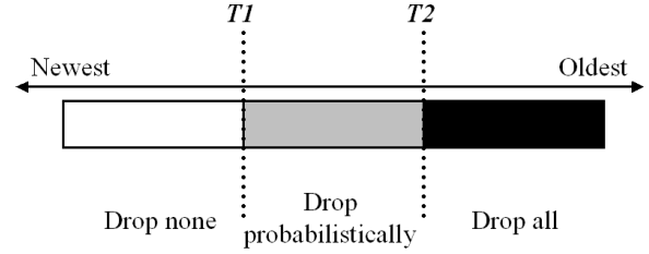
Figure 2. Sorted List of Active Transaction Contexts
