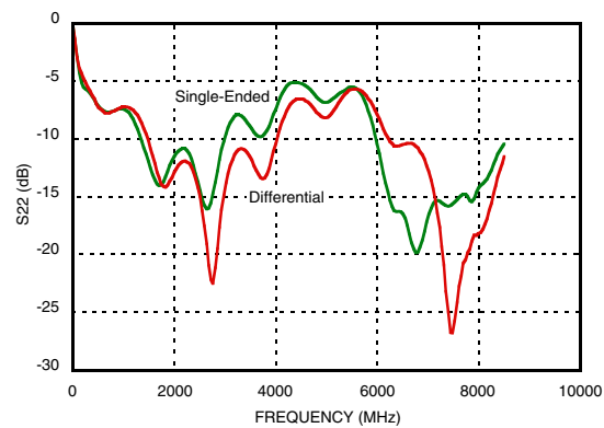
Figure 22. S-Parameters - S22 [11]
