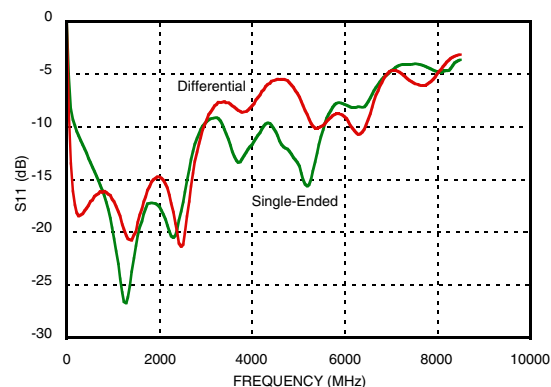
Figure 20. S-Parameters - S11 [11]
